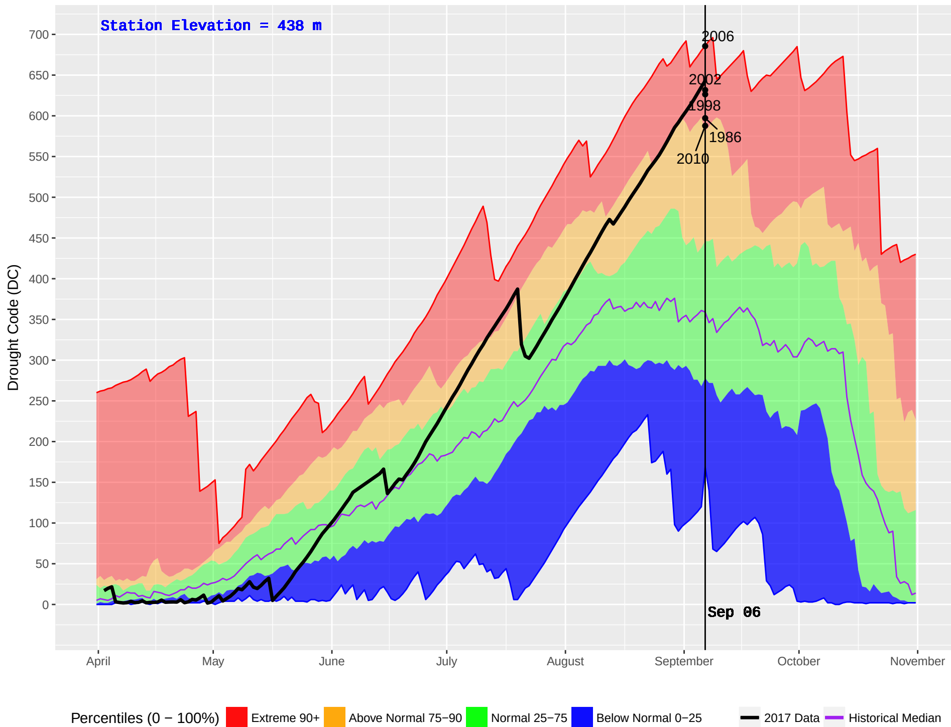
MENZIES CAMP (19) : Historical (1970–2016) and Current (2017) Noon Drought Code (DC)
